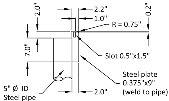
ANCHORAGE
