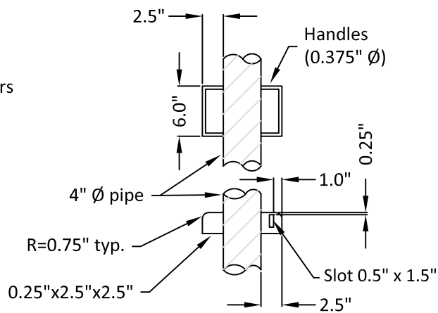
POST
