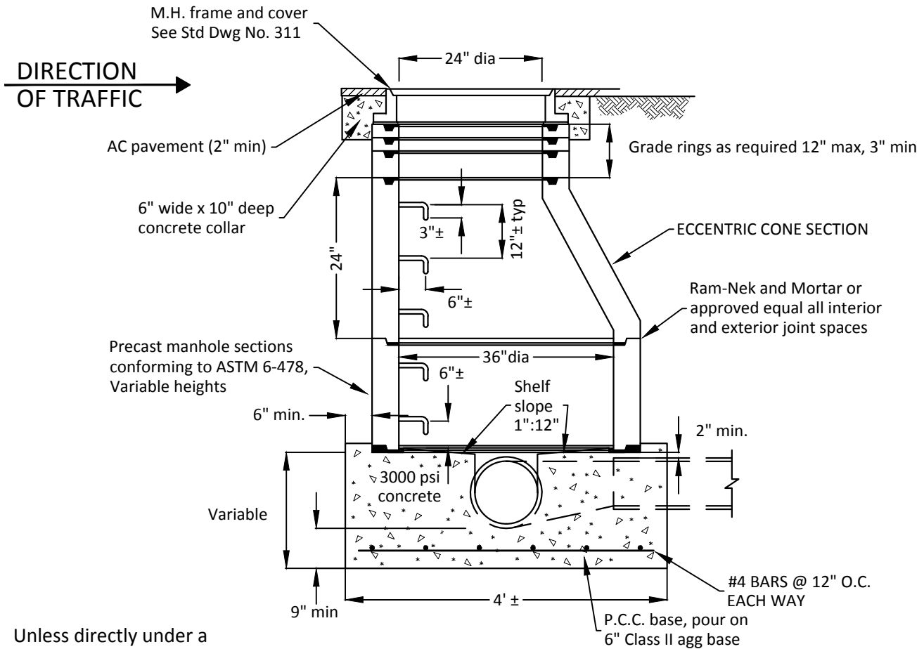
SECTION
