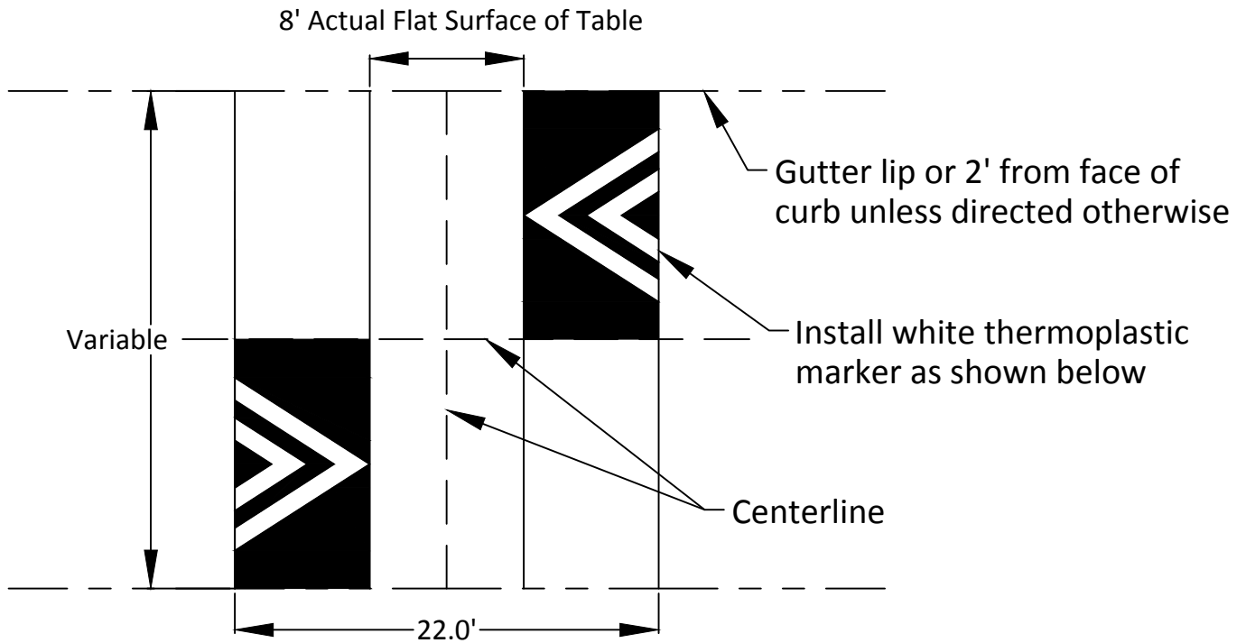
Typical Speed Table Plan
