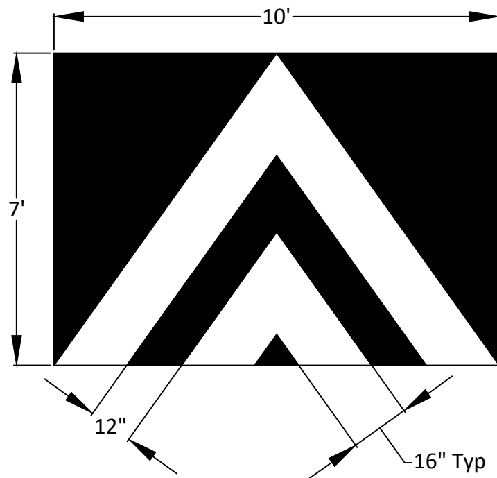
Typical White Triangular Bump Marker
