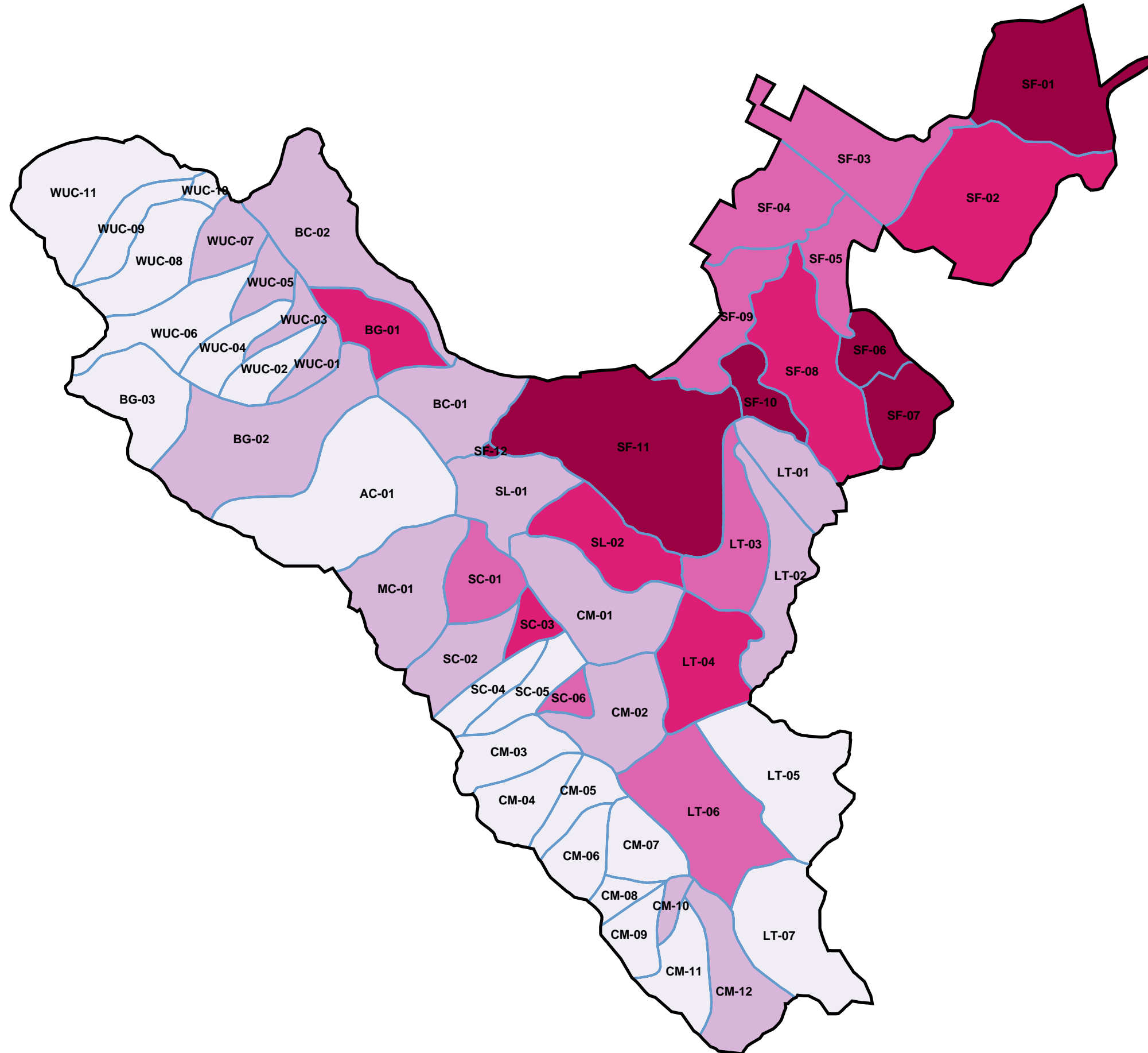
Figure 16 Human - related Erosion as a Percentage of Total Erosion in the San Francisquito Watershed
