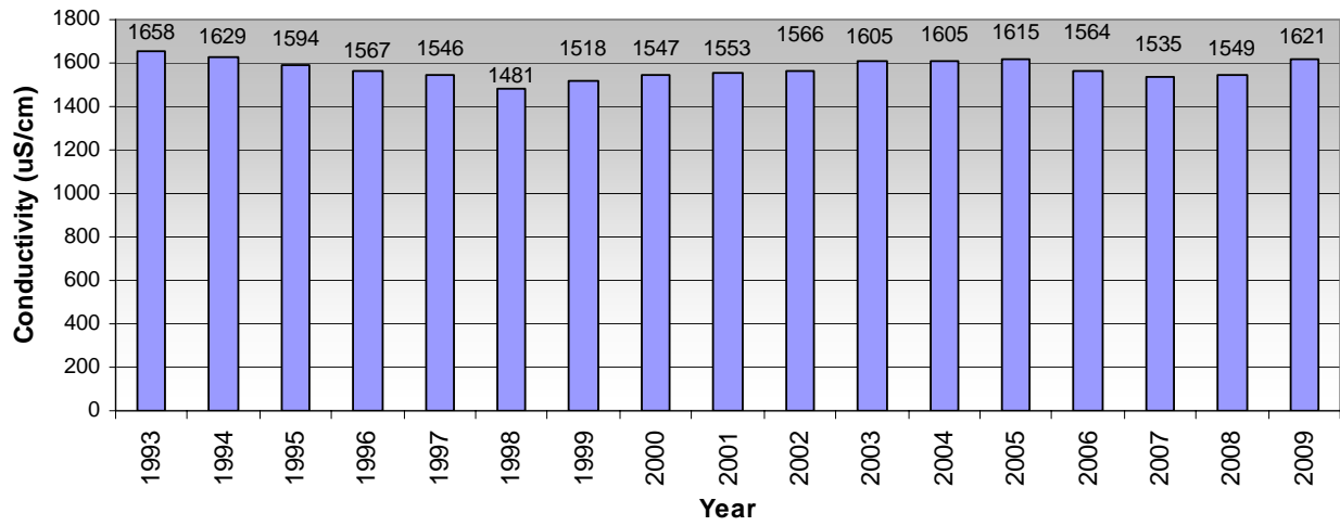
RWQCP Influent Annual Average Conductivity: 1993 - 2009
