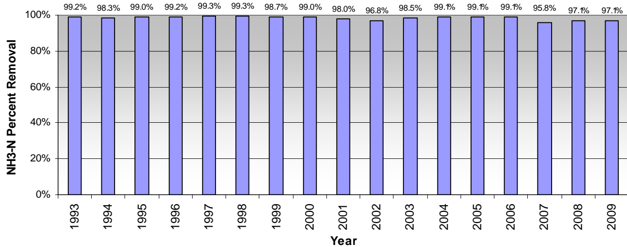
RWQCP Annual Average NH3-N Percent Removal: 1993 - 2009
