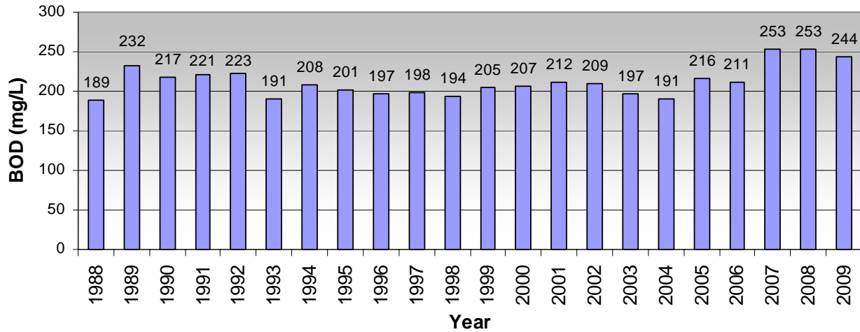
RWQCP Influent Annual Average BOD: 1988 - 2009
