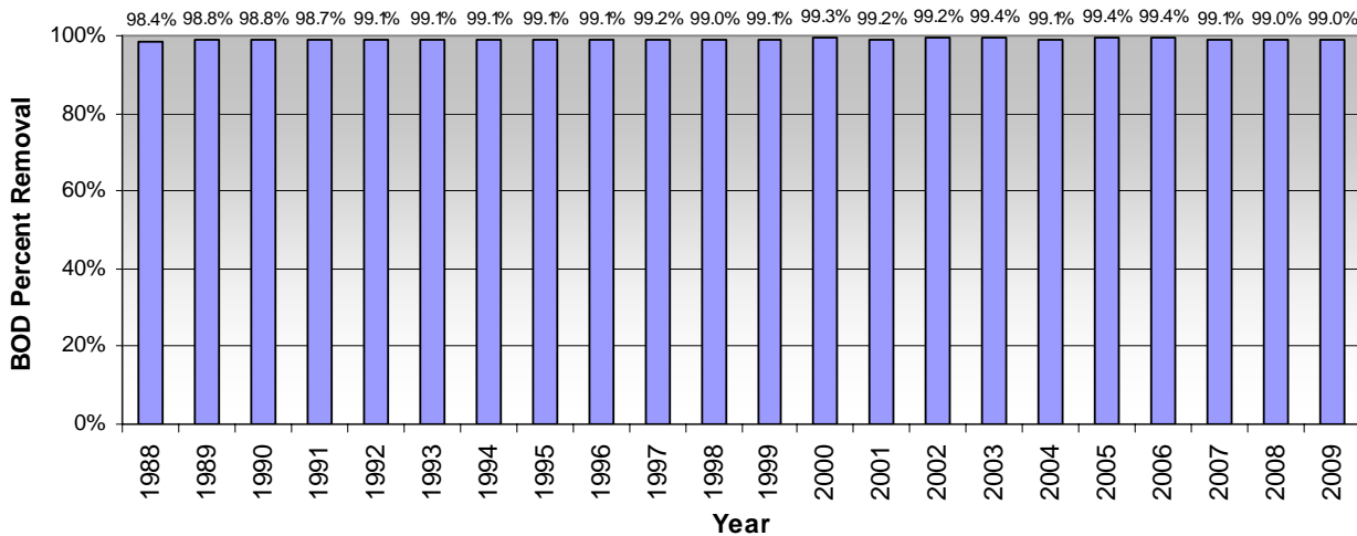
RWQCP Annual Average BOD Percent Removal: 1988 - 2009
