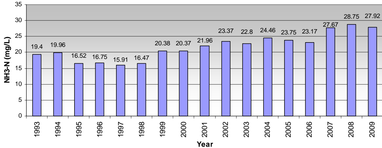
RWQCP Influent Annual Average NH3-N: 1993 - 2009
