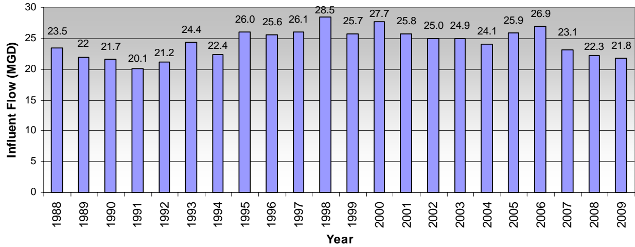
RWQCP Influent Annual Average Daily Flow: 1988 - 2009
