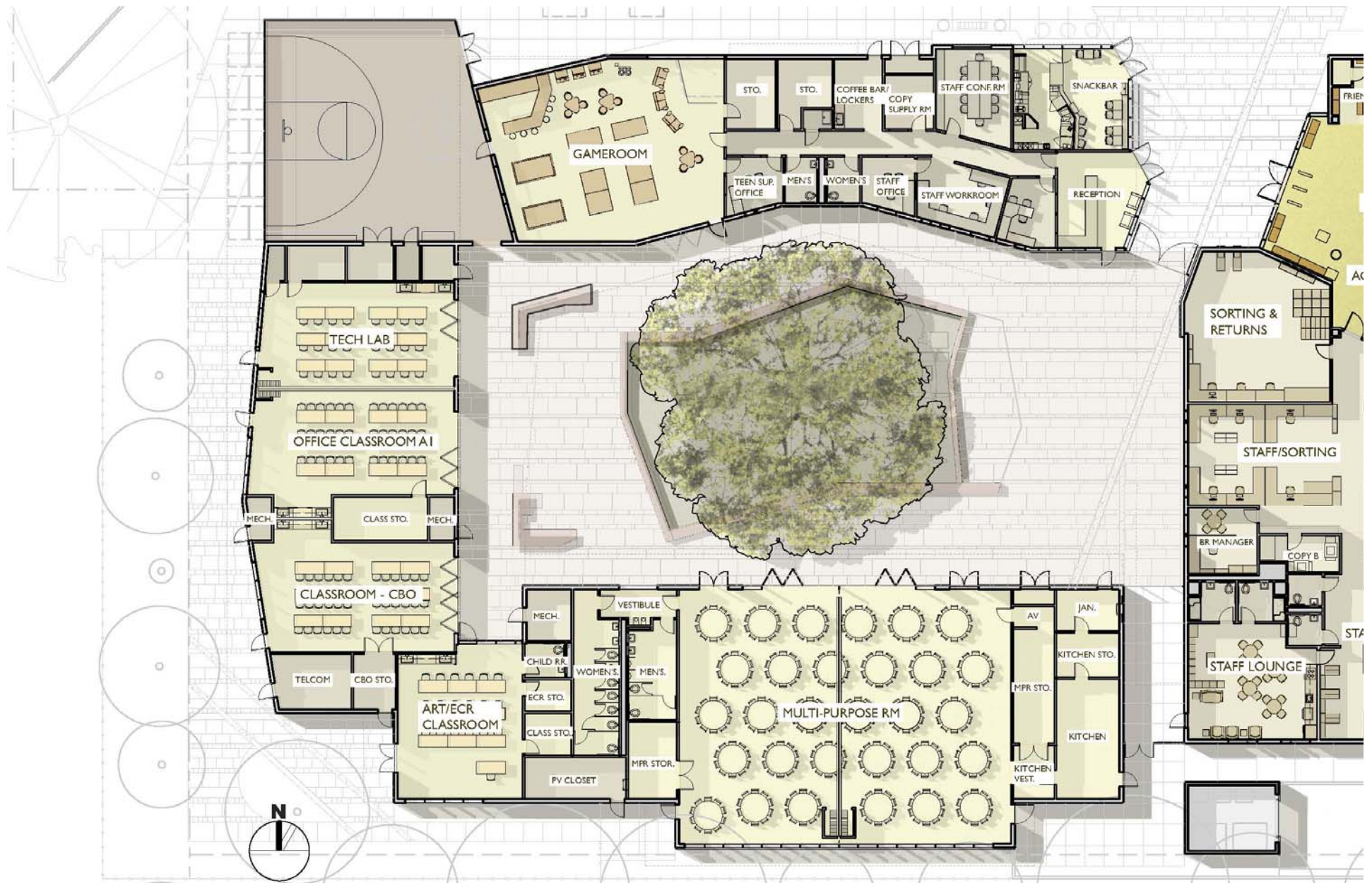
MITCHELL PARK Community Center First Floor Plan
