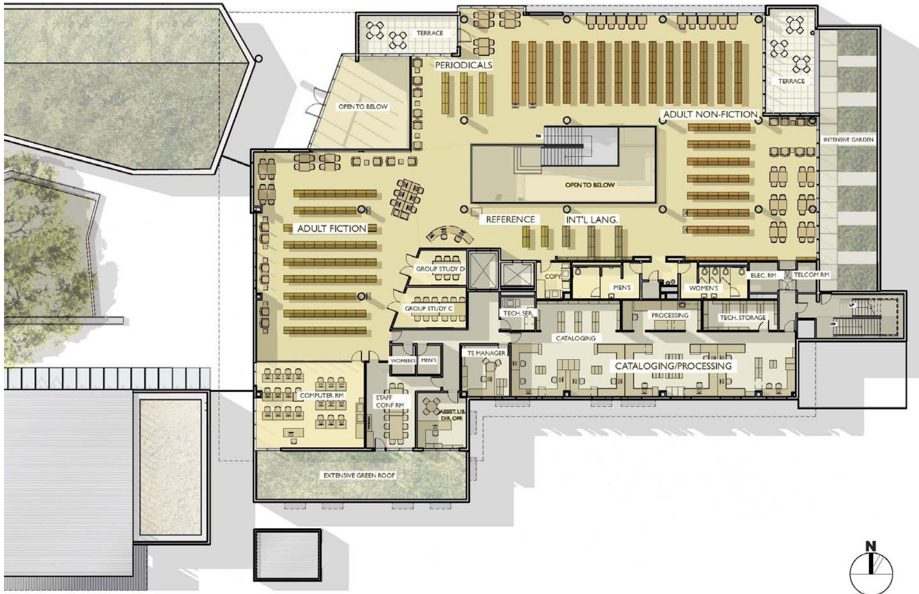
MITCHELL PARK Library Second Floor Plan
