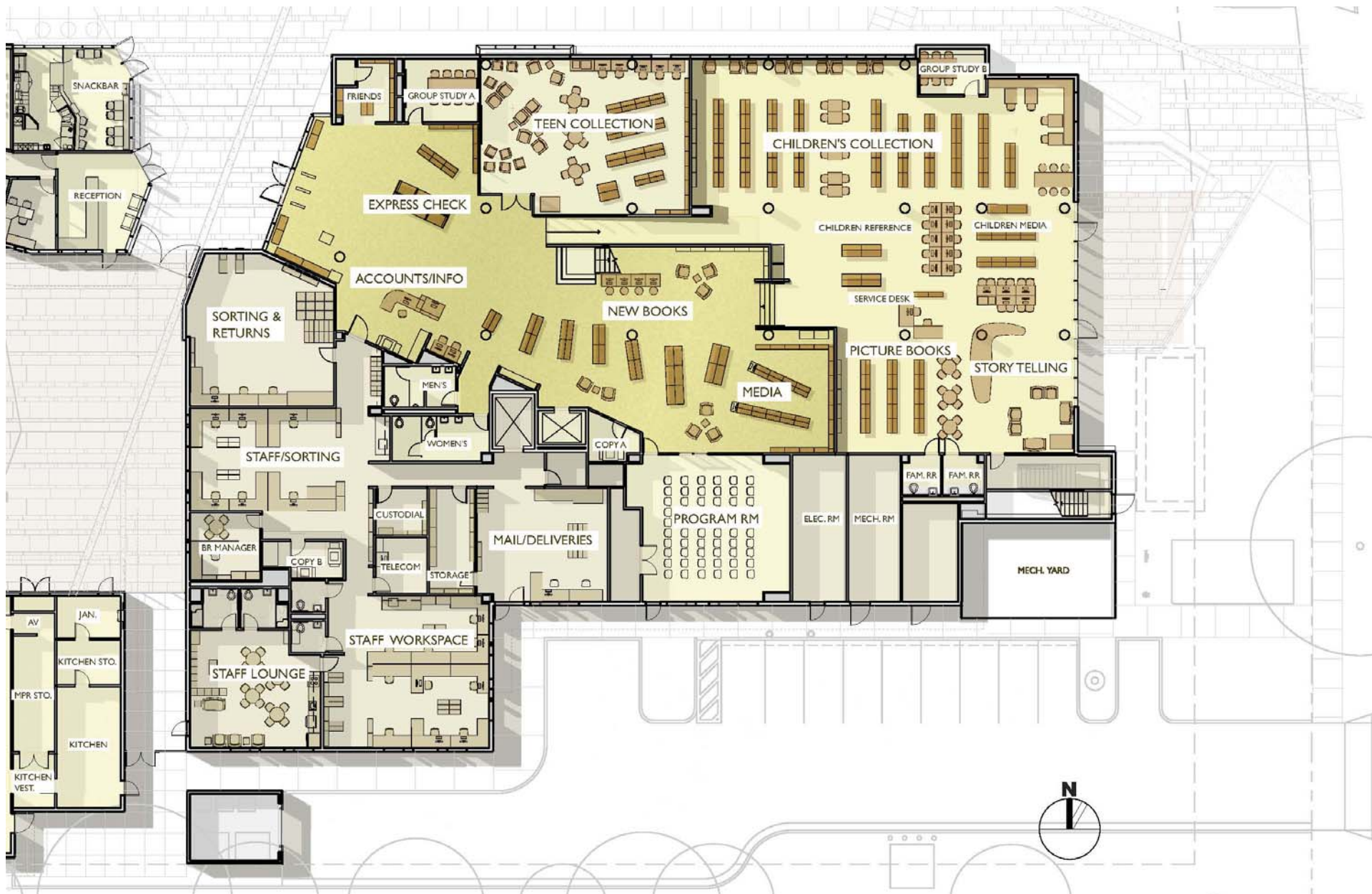
MITCHELL PARK Library First Floor Plan
